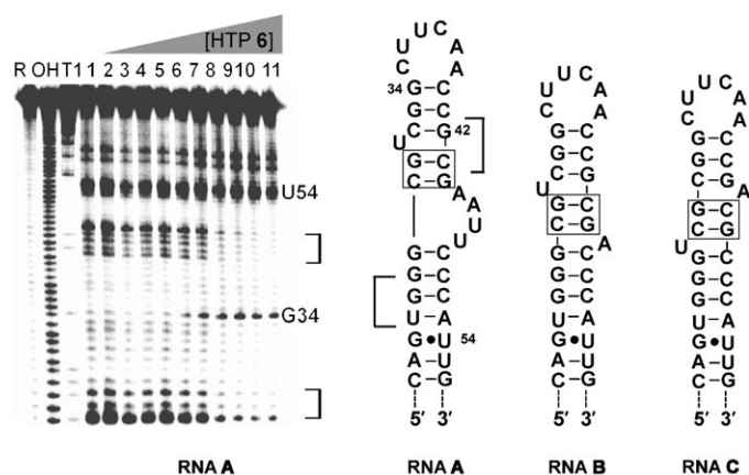
Figure 1. Left: Quantitative ribonuclease V1 footprinting of HTP 6 binding to RNA A . Lane R: RNA alone, lane OH: alkaline hydrolysis, lane T1: ribonuclease T1 products (G lane), lanes 1–11: ribonuclease V1 products. Lane 1: no HTP, lanes 2–11: [HTP 6 ] = 1 nM, 3 nM, 10 nM, 30 nM, 100 nM, 300 nM, 1 \mu M, 3 \mu M, 10 \mu M, 30 \mu M, respectively. Right: Structures of RNA molecules A , B , and C used in this study with the putative intercalation sites indicated with a box.
